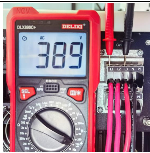
Line voltage(line voltage= \sqrt{3} ×Phase voltage)
